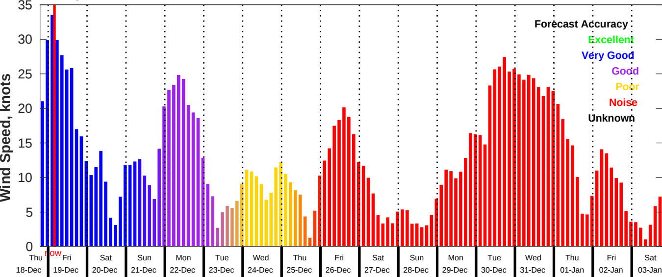
GFS Wind Speed Forecast for NDBC 41013 from 18-Dec-2025 19:00:00 to 03-Jan-2026 19:00:00
