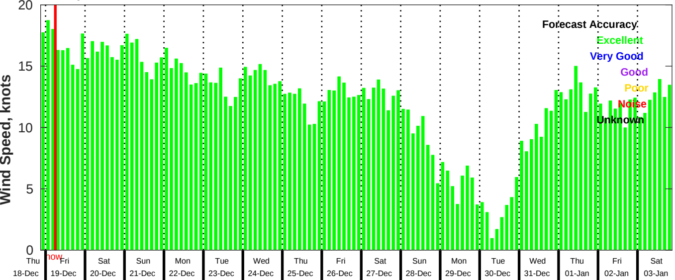
GFS Wind Speed Forecast for NDBC 41040 from 18-Dec-2025 21:00:00 to 03-Jan-2026 21:00:00
