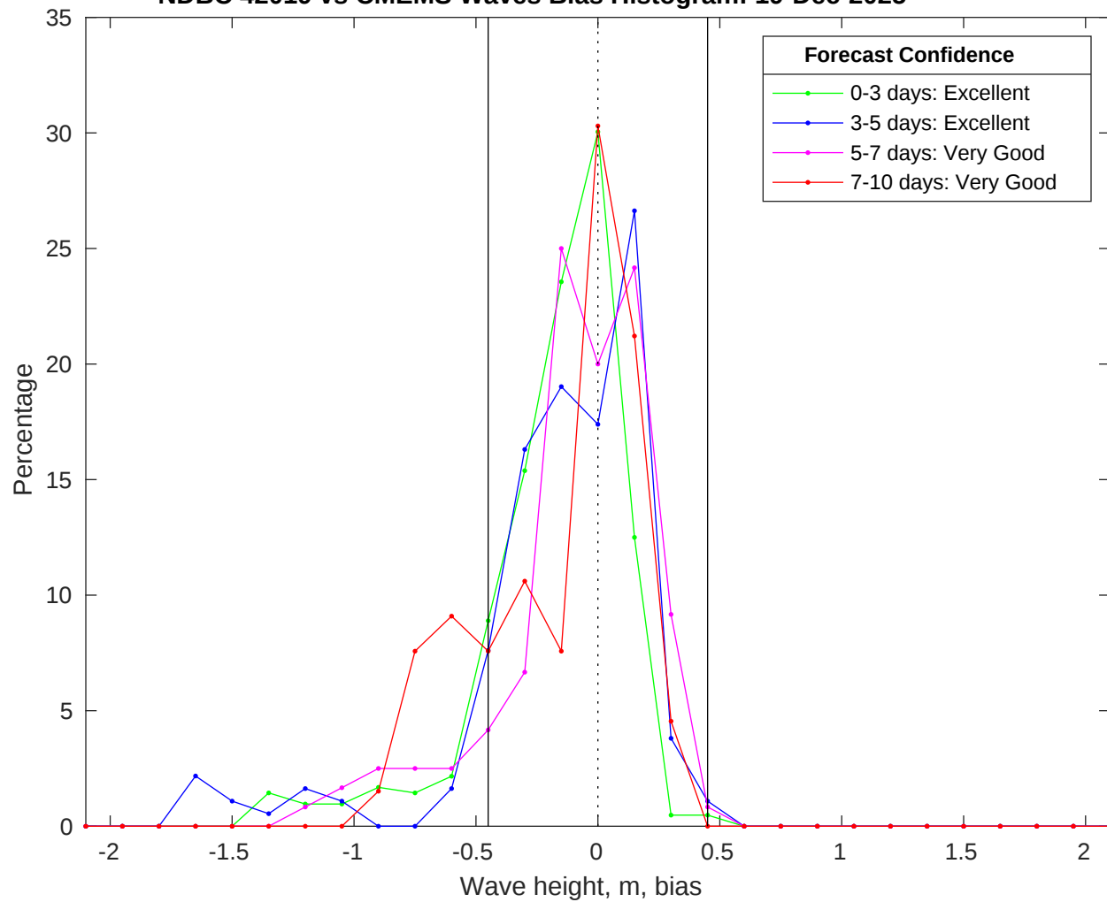
NDBC 42019 vs CMEMS Waves Bias Histogram: 19-Dec-2025
