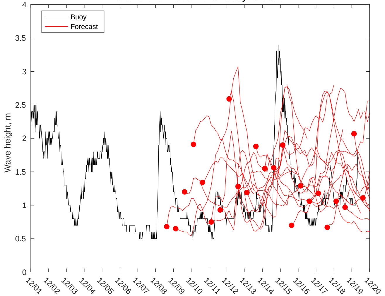
NDBC 42019 vs GFS Waves: 10 to 16 day forecast
