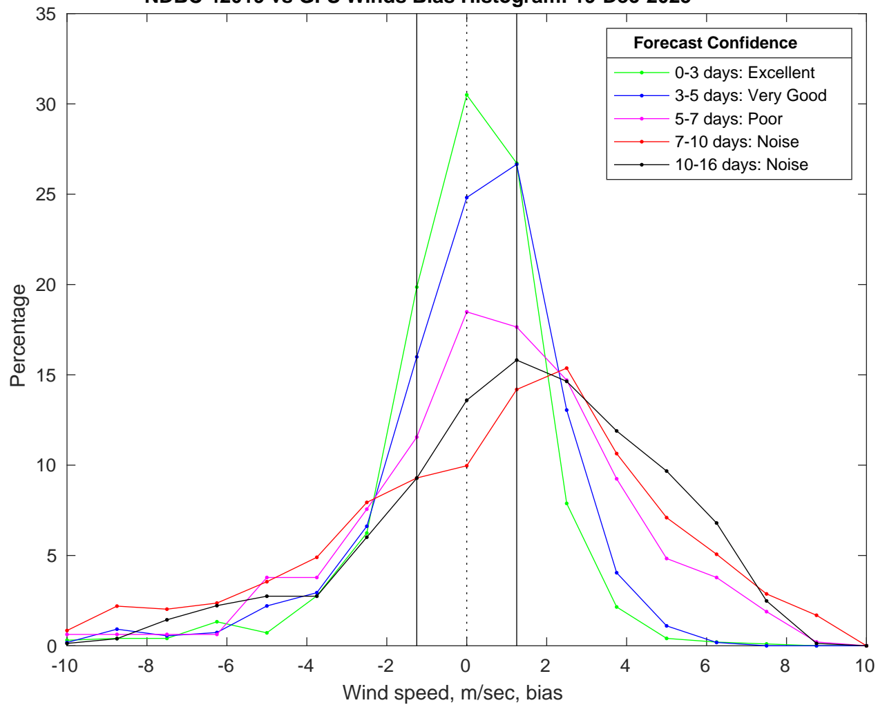
NDBC 42019 vs GFS Winds Bias Histogram: 19-Dec-2025
