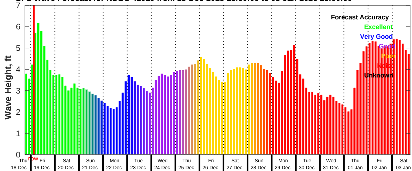
GFS Wave Forecast for NDBC 42019 from 18-Dec-2025 18:00:00 to 03-Jan-2026 18:00:00
