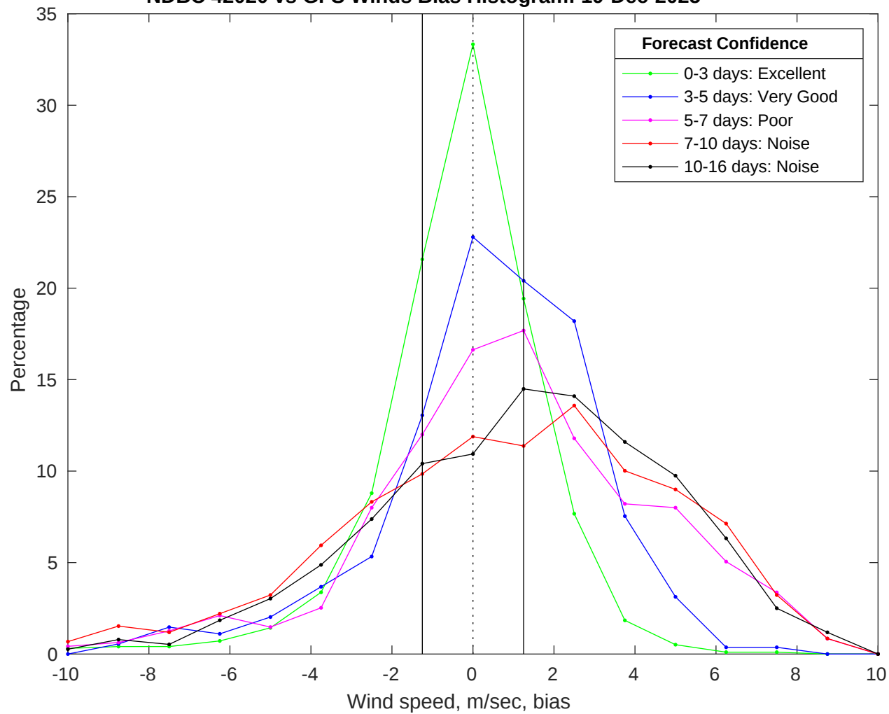
NDBC 42020 vs GFS Winds Bias Histogram: 19-Dec-2025
