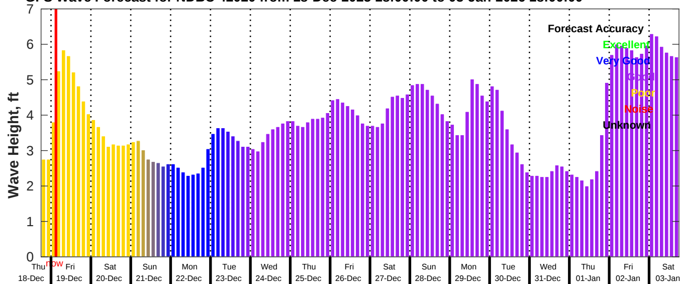
GFS Wave Forecast for NDBC 42020 from 18-Dec-2025 18:00:00 to 03-Jan-2026 18:00:00
