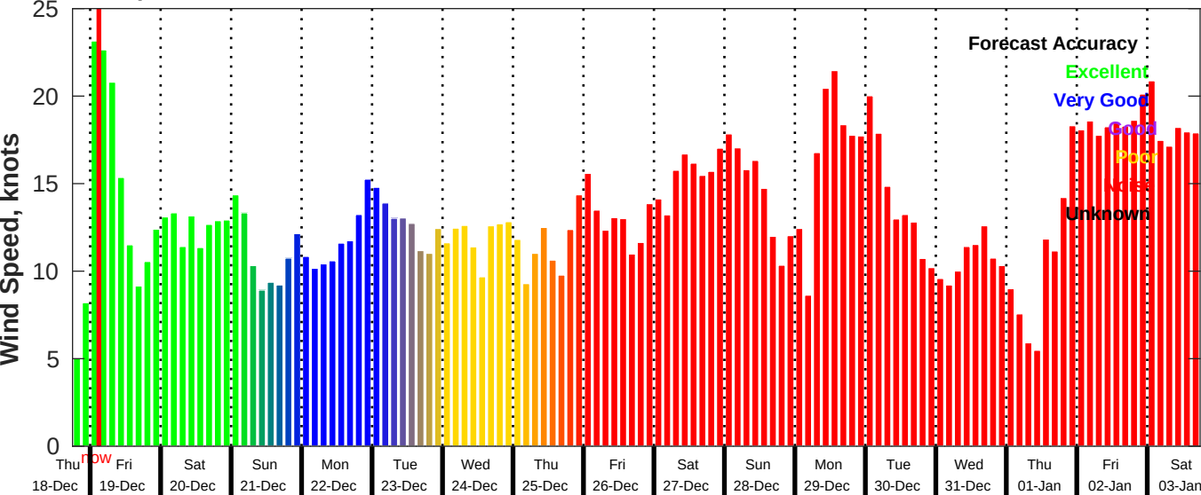
GFS Wind Speed Forecast for NDBC 42020 from 18-Dec-2025 18:00:00 to 03-Jan-2026 18:00:00
