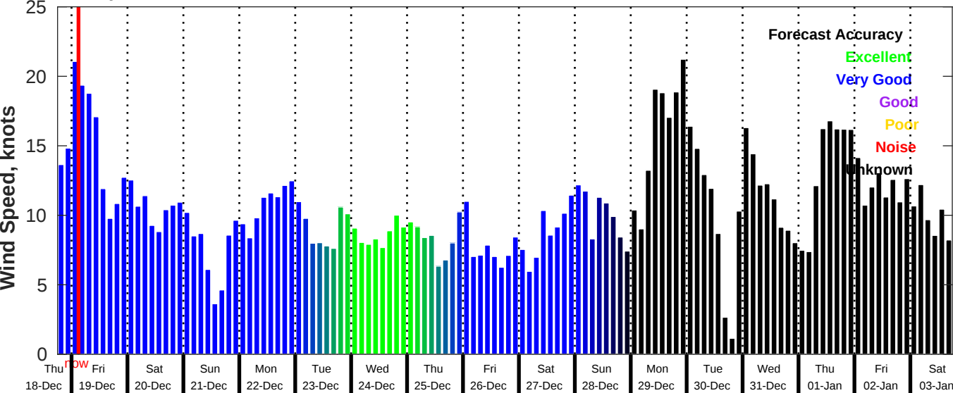
GFS Wind Speed Forecast for NDBC 42035 from 18-Dec-2025 18:00:00 to 03-Jan-2026 18:00:00
