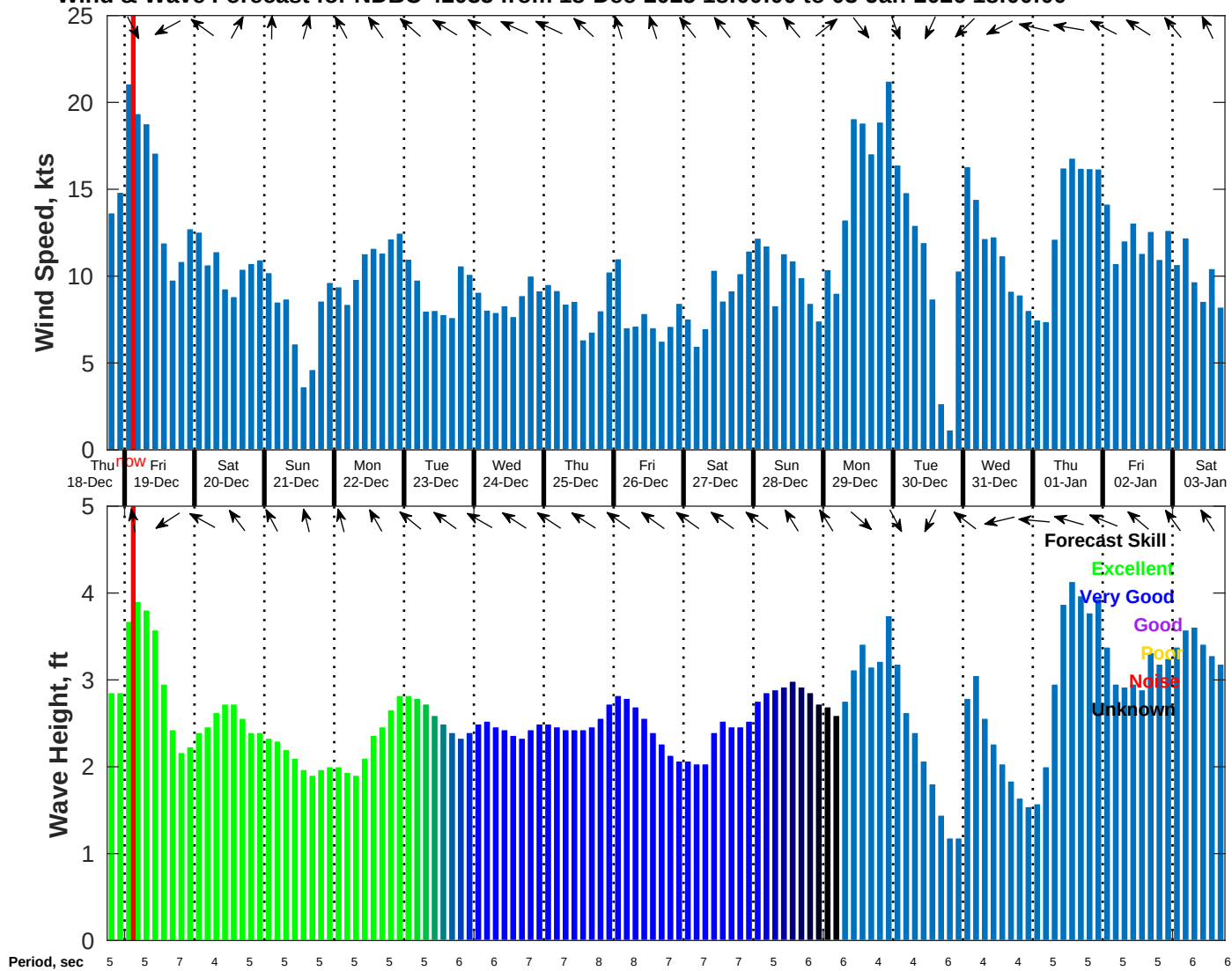
Wind & Wave Forecast for NDBC 42035 from 18-Dec-2025 18:00:00 to 03-Jan-2026 18:00:00
