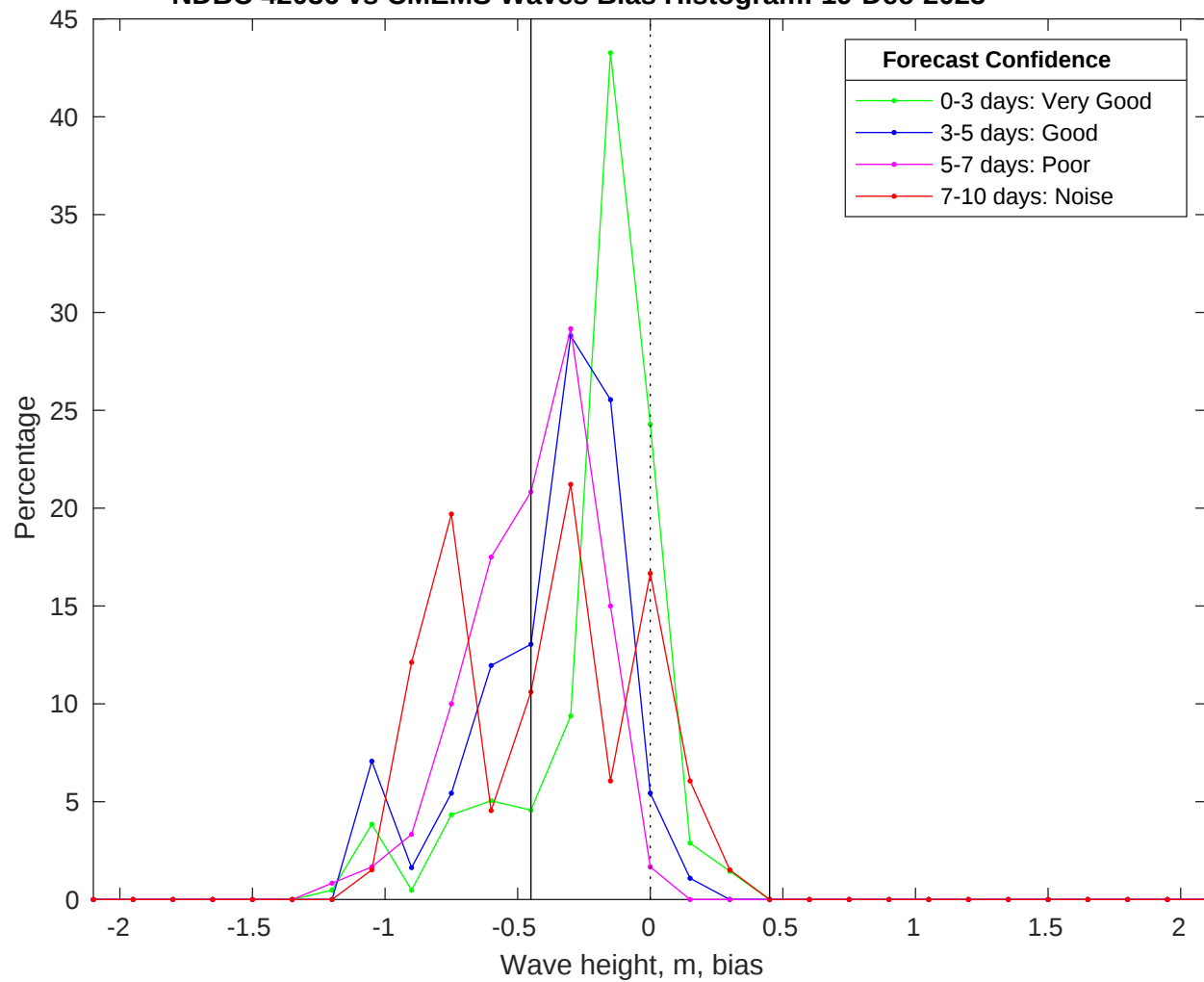
NDBC 42036 vs CMEMS Waves Bias Histogram: 19-Dec-2025
