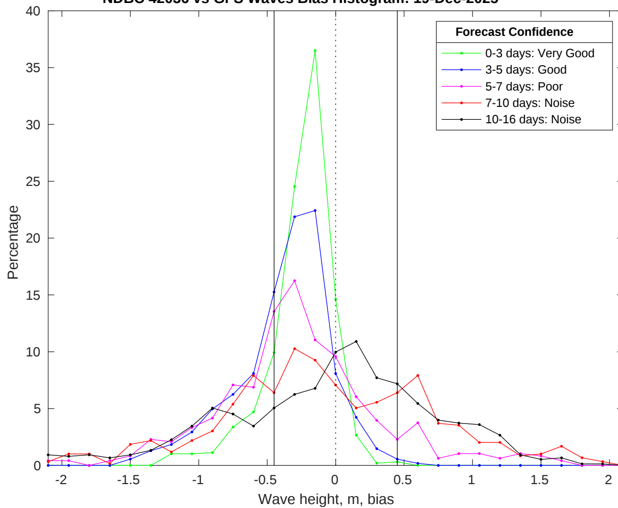
NDBC 42036 vs GFS Waves Bias Histogram: 19-Dec-2025
