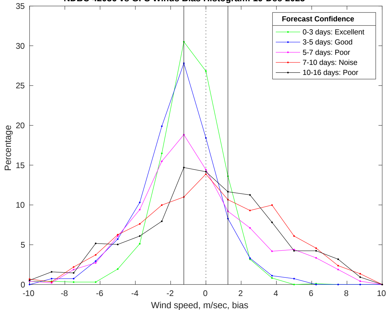
NDBC 42036 vs GFS Winds Bias Histogram: 19-Dec-2025
