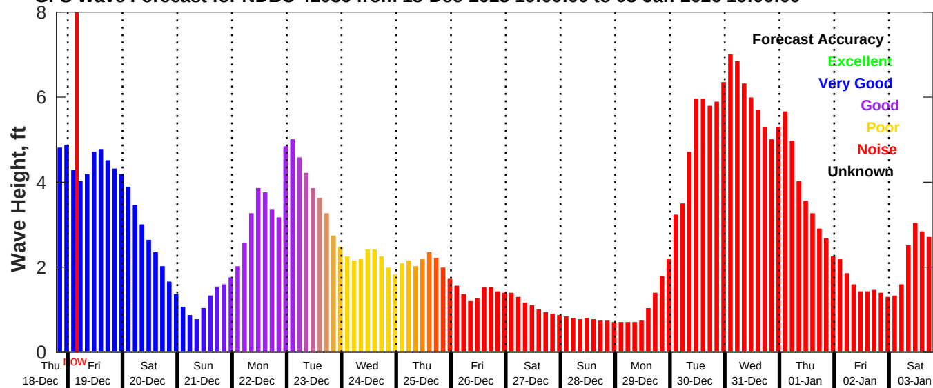
GFS Wave Forecast for NDBC 42036 from 18-Dec-2025 19:00:00 to 03-Jan-2026 19:00:00
