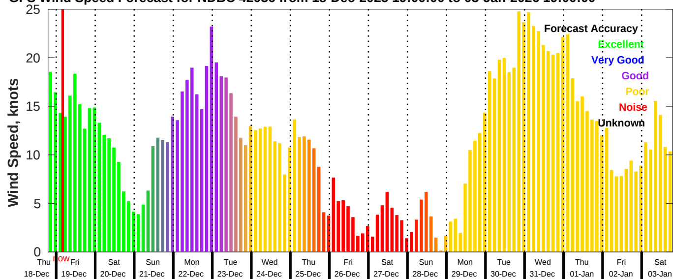
GFS Wind Speed Forecast for NDBC 42036 from 18-Dec-2025 19:00:00 to 03-Jan-2026 19:00:00
