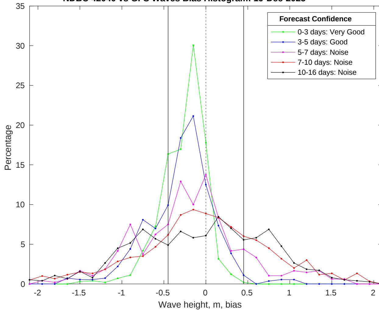
NDBC 42040 vs GFS Waves Bias Histogram: 19-Dec-2025
