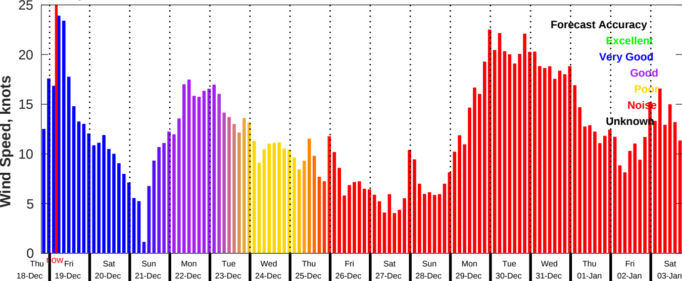
GFS Wind Speed Forecast for NDBC 42040 from 18-Dec-2025 19:00:00 to 03-Jan-2026 19:00:00
