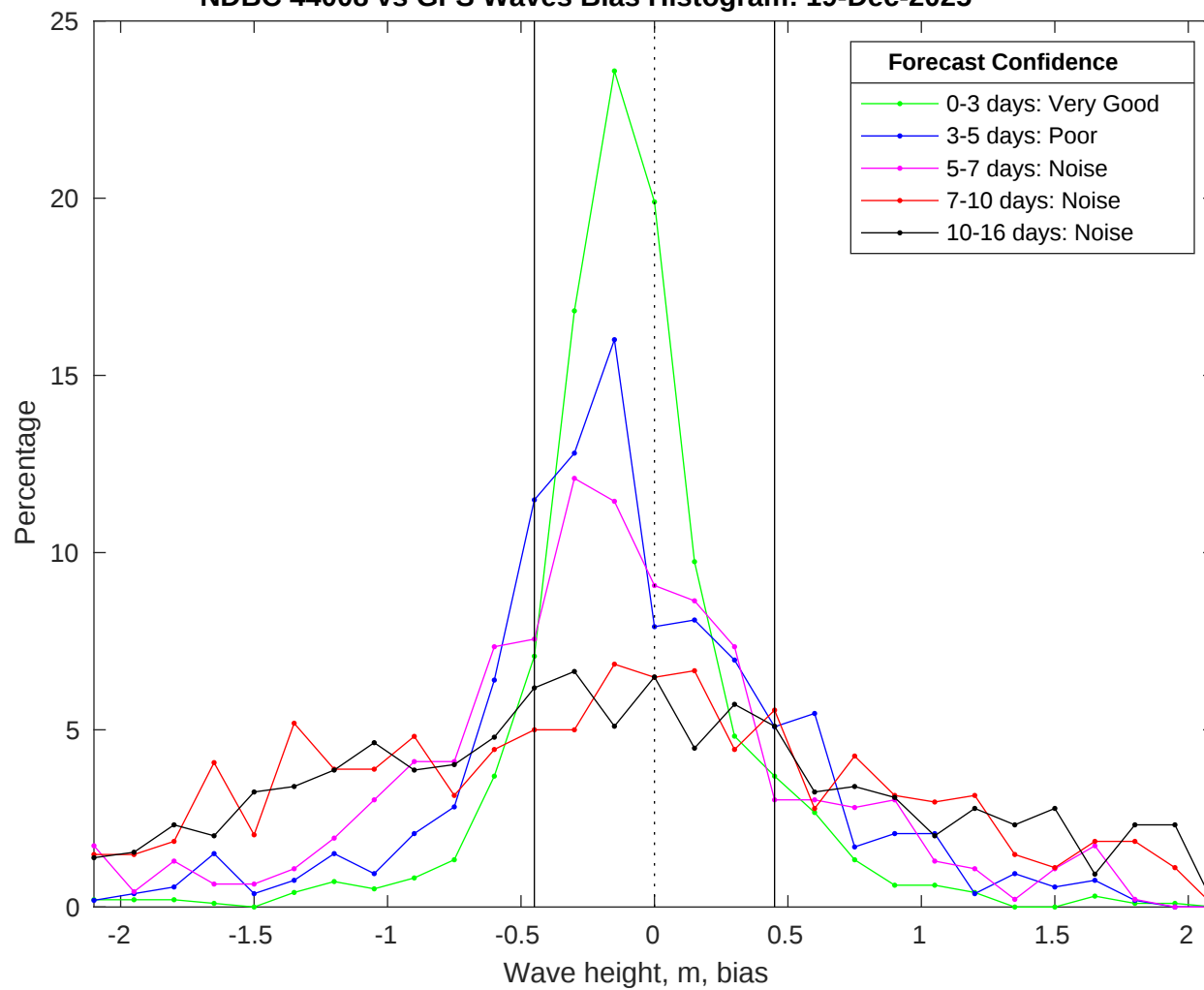
NDBC 44008 vs GFS Waves Bias Histogram: 19-Dec-2025
