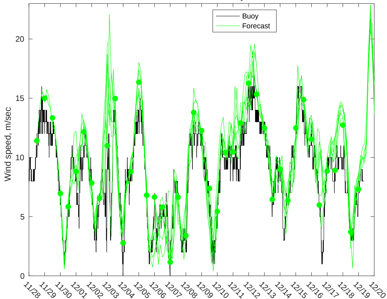
NDBC 44008 vs GFS Winds: 0 to 3 day forecast
