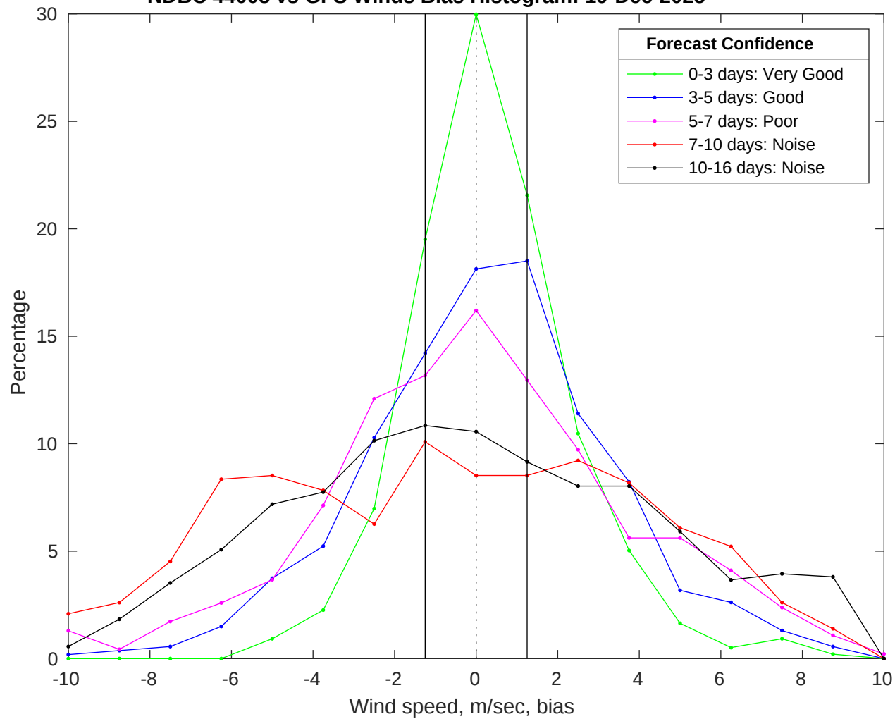
NDBC 44008 vs GFS Winds Bias Histogram: 19-Dec-2025
