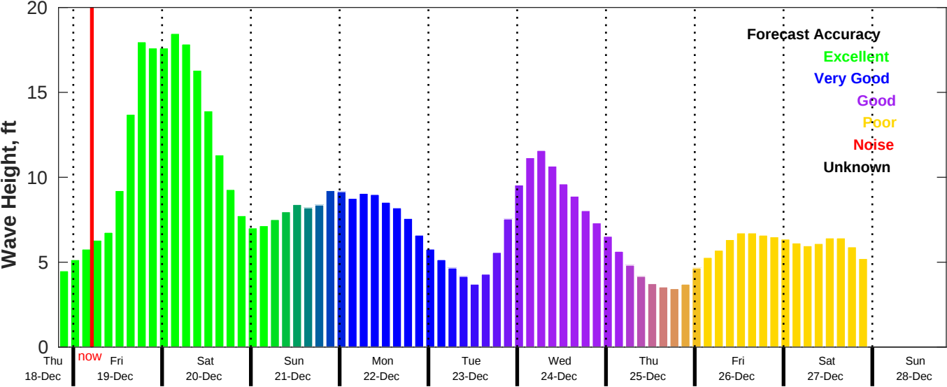
CMEMS Wave Forecast for NDBC 44008 from 18-Dec-2025 20:00:00 to 28-Dec-2025 20:00:00
