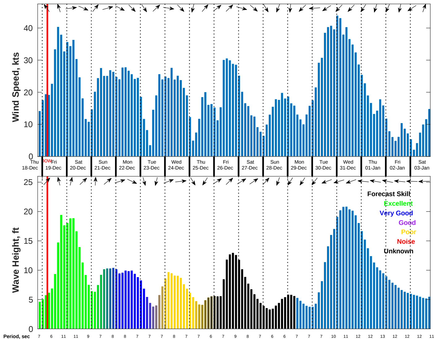
Wind & Wave Forecast for NDBC 44008 from 18-Dec-2025 20:00:00 to 03-Jan-2026 20:00:00
