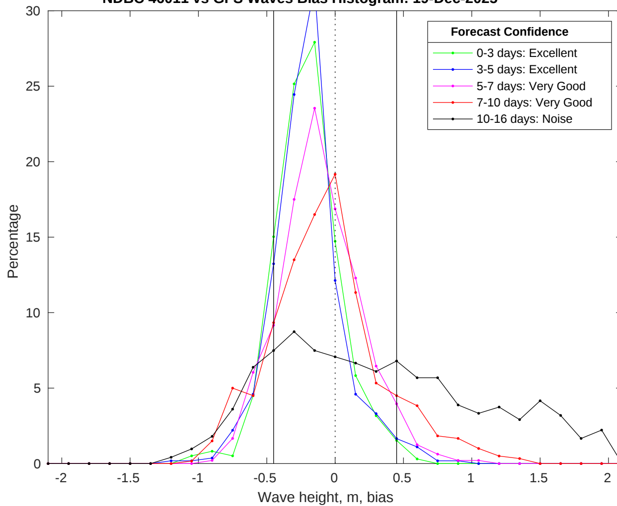
NDBC 46011 vs GFS Waves Bias Histogram: 19-Dec-2025
