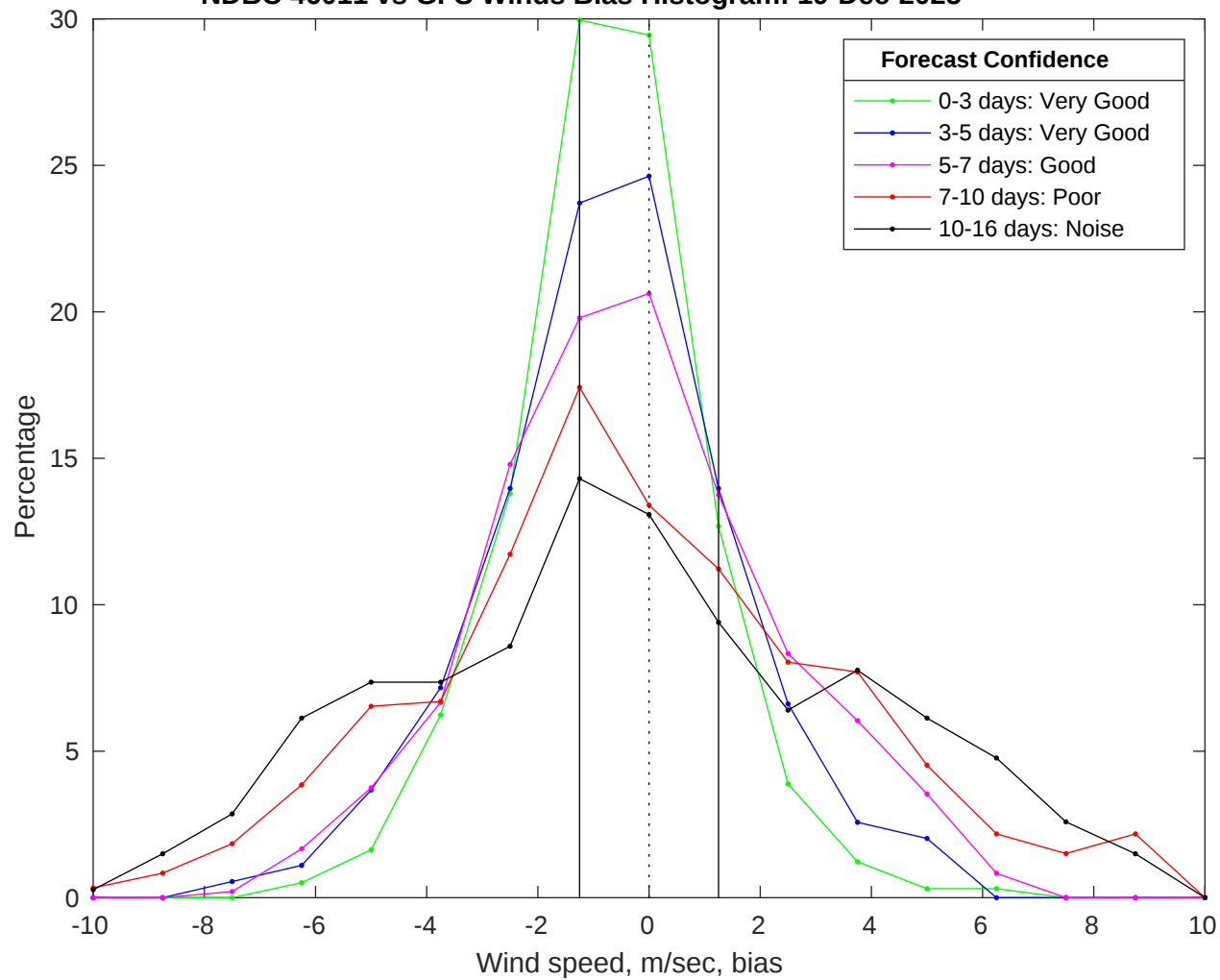
NDBC 46011 vs GFS Winds Bias Histogram: 19-Dec-2025
