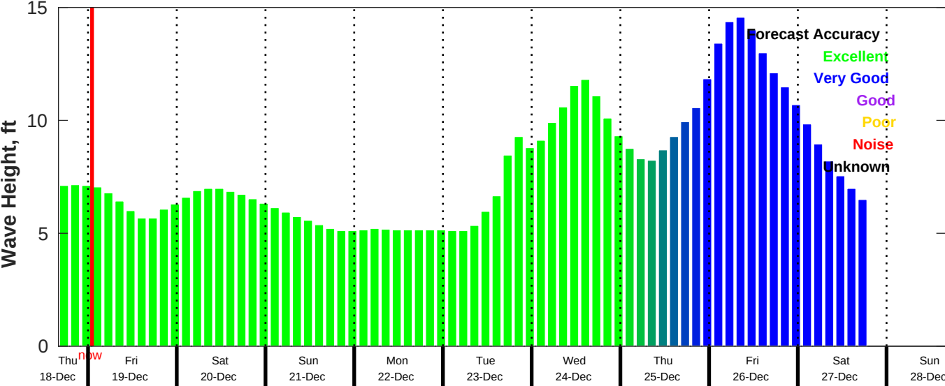
CMEMS Wave Forecast for NDBC 46011 from 18-Dec-2025 16:00:00 to 28-Dec-2025 16:00:00
