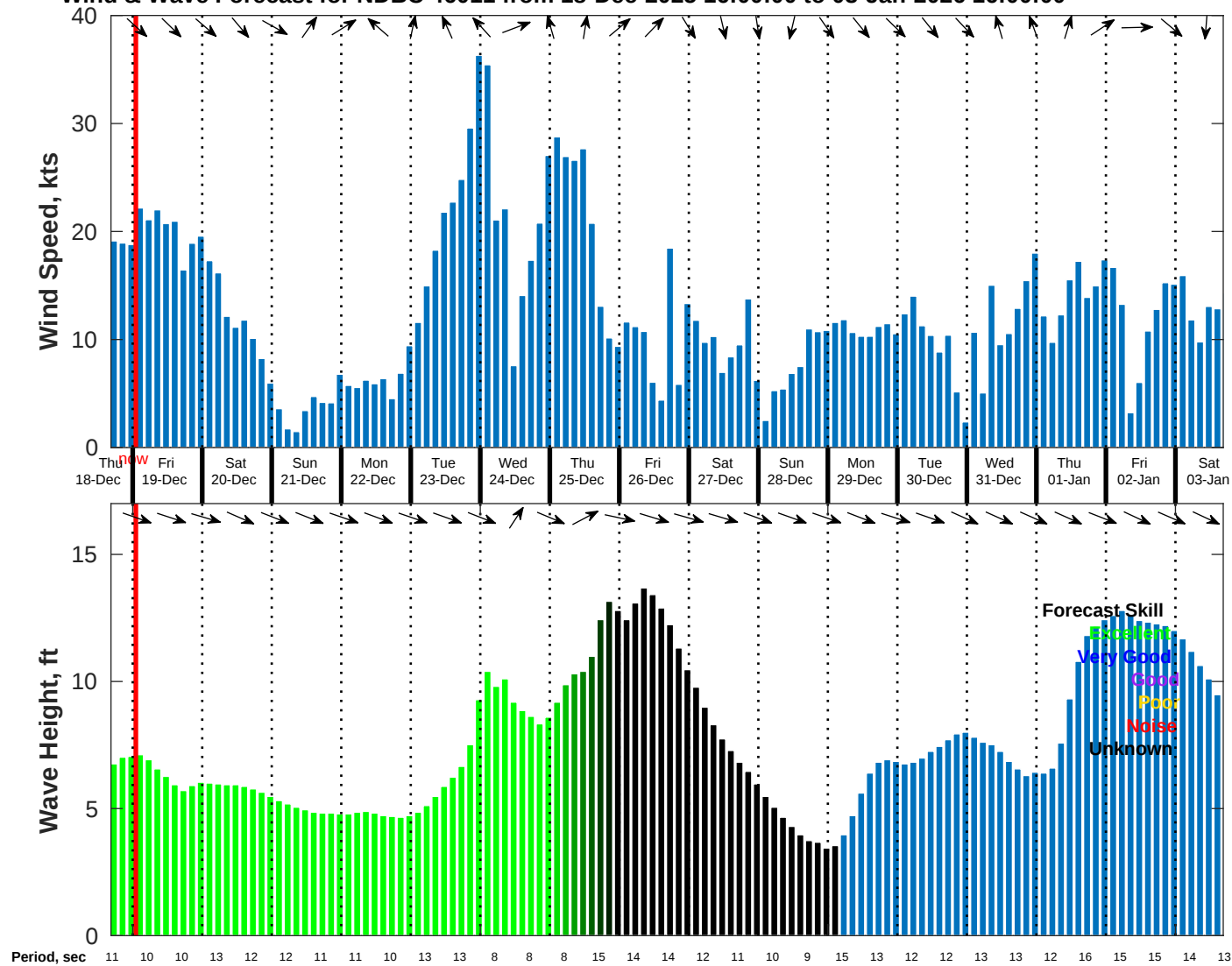
Wind & Wave Forecast for NDBC 46011 from 18-Dec-2025 16:00:00 to 03-Jan-2026 16:00:00
