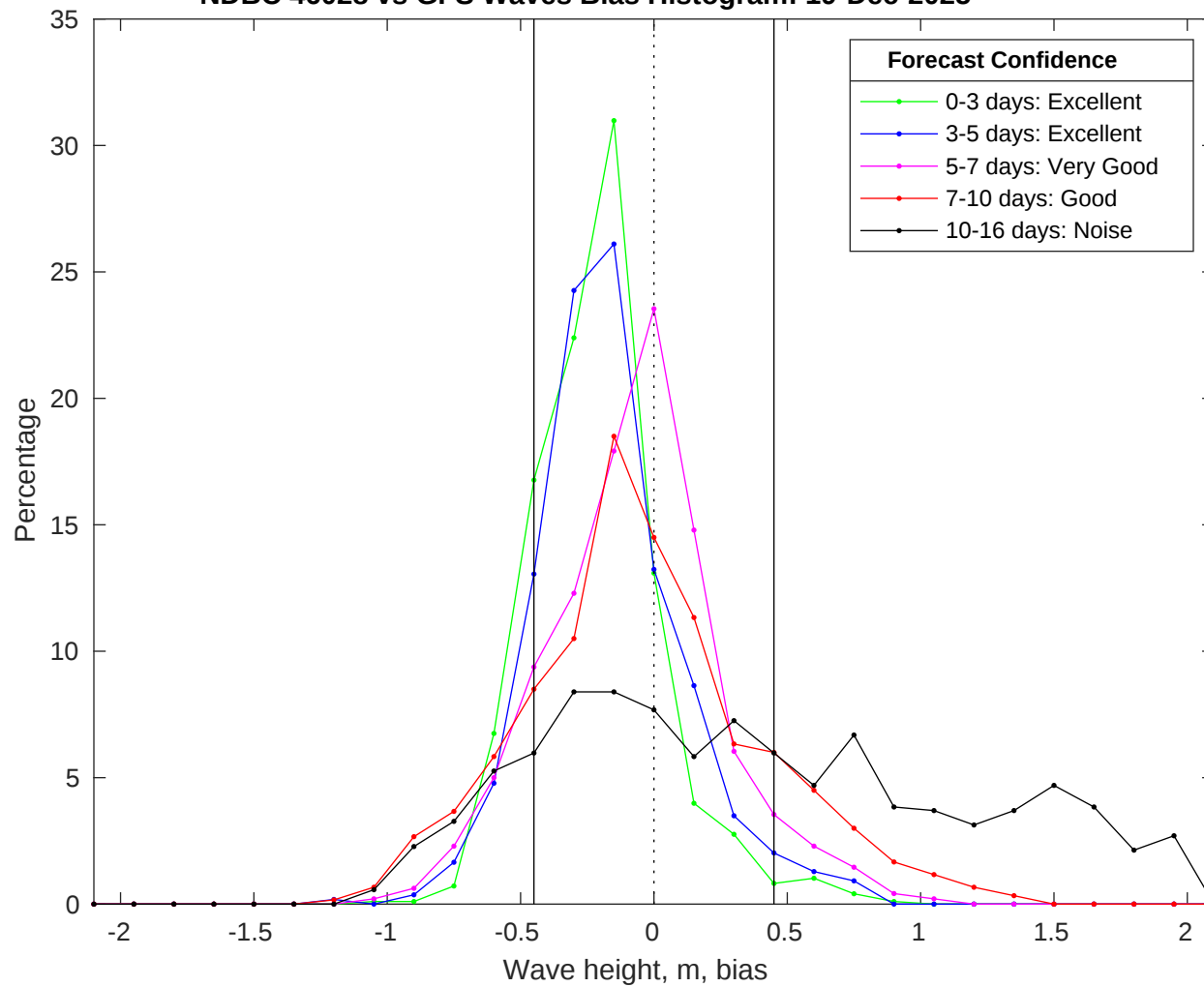
NDBC 46028 vs GFS Waves Bias Histogram: 19-Dec-2025
