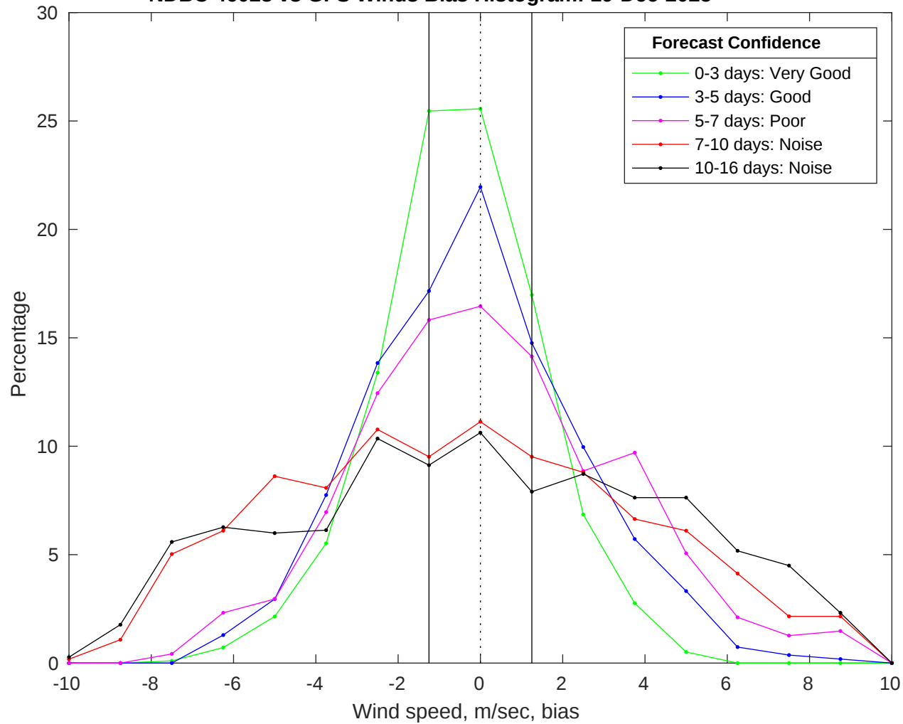
NDBC 46028 vs GFS Winds Bias Histogram: 19-Dec-2025
