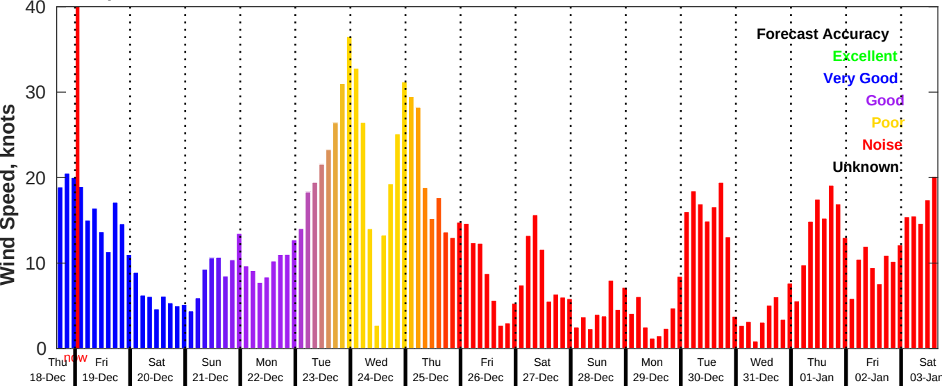
GFS Wind Speed Forecast for NDBC 46028 from 18-Dec-2025 16:00:00 to 03-Jan-2026 16:00:00
