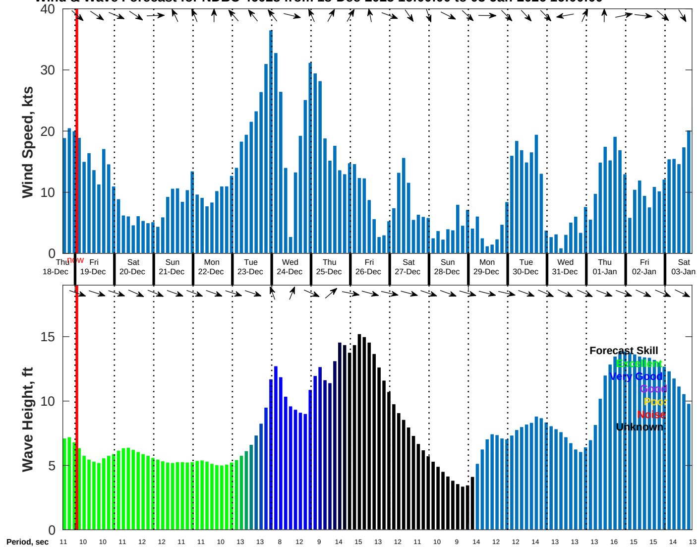
Wind & Wave Forecast for NDBC 46028 from 18-Dec-2025 16:00:00 to 03-Jan-2026 16:00:00
