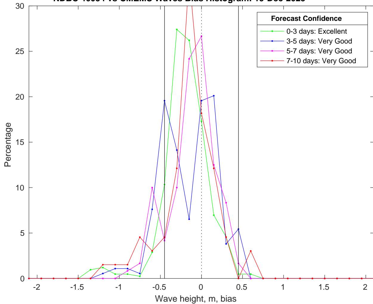
NDBC 46054 vs CMEMS Waves Bias Histogram: 19-Dec-2025
