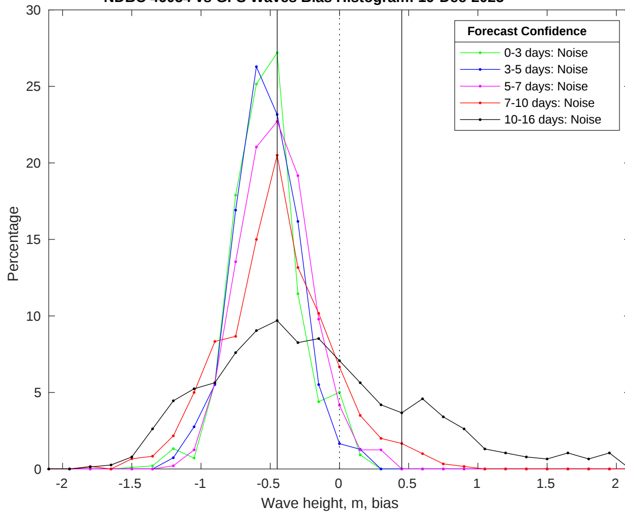
NDBC 46054 vs GFS Waves Bias Histogram: 19-Dec-2025
