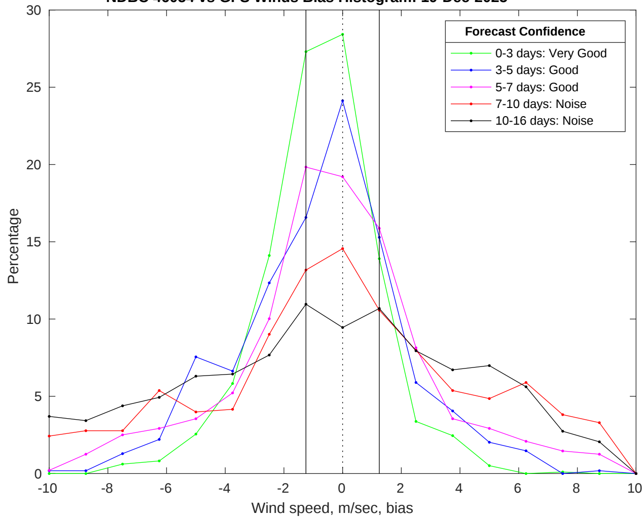
NDBC 46054 vs GFS Winds Bias Histogram: 19-Dec-2025
