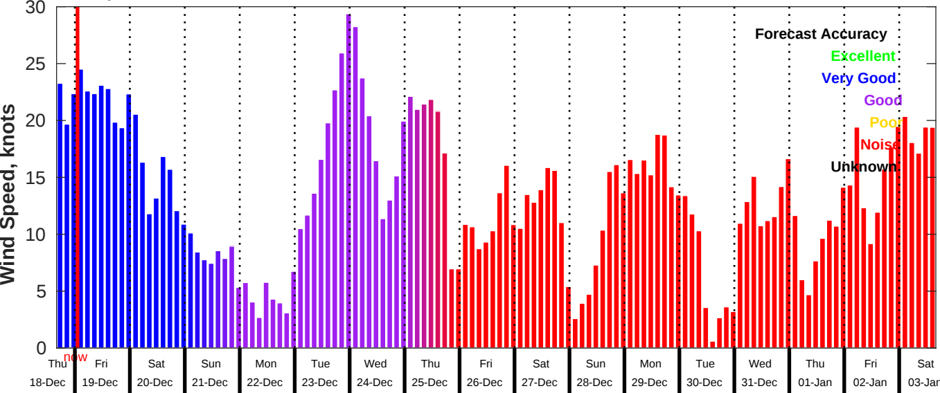
GFS Wind Speed Forecast for NDBC 46054 from 18-Dec-2025 16:00:00 to 03-Jan-2026 16:00:00
