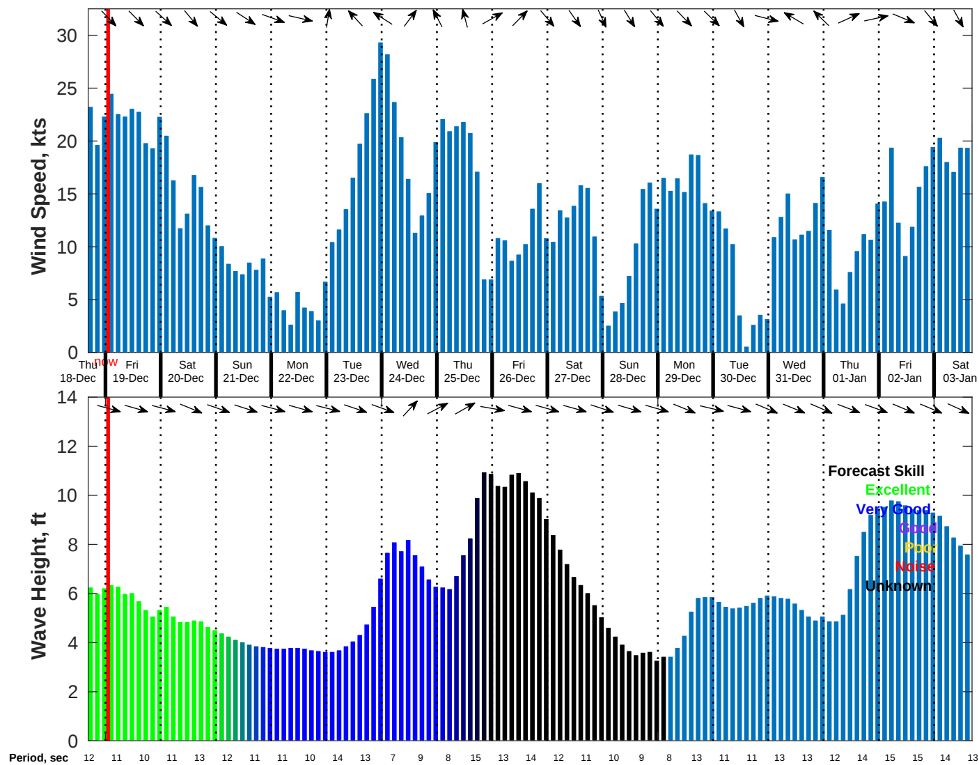
Wind & Wave Forecast for NDBC 46054 from 18-Dec-2025 16:00:00 to 03-Jan-2026 16:00:00
