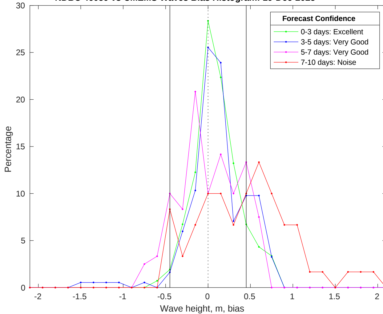
NDBC 46059 vs CMEMS Waves Bias Histogram: 19-Dec-2025
