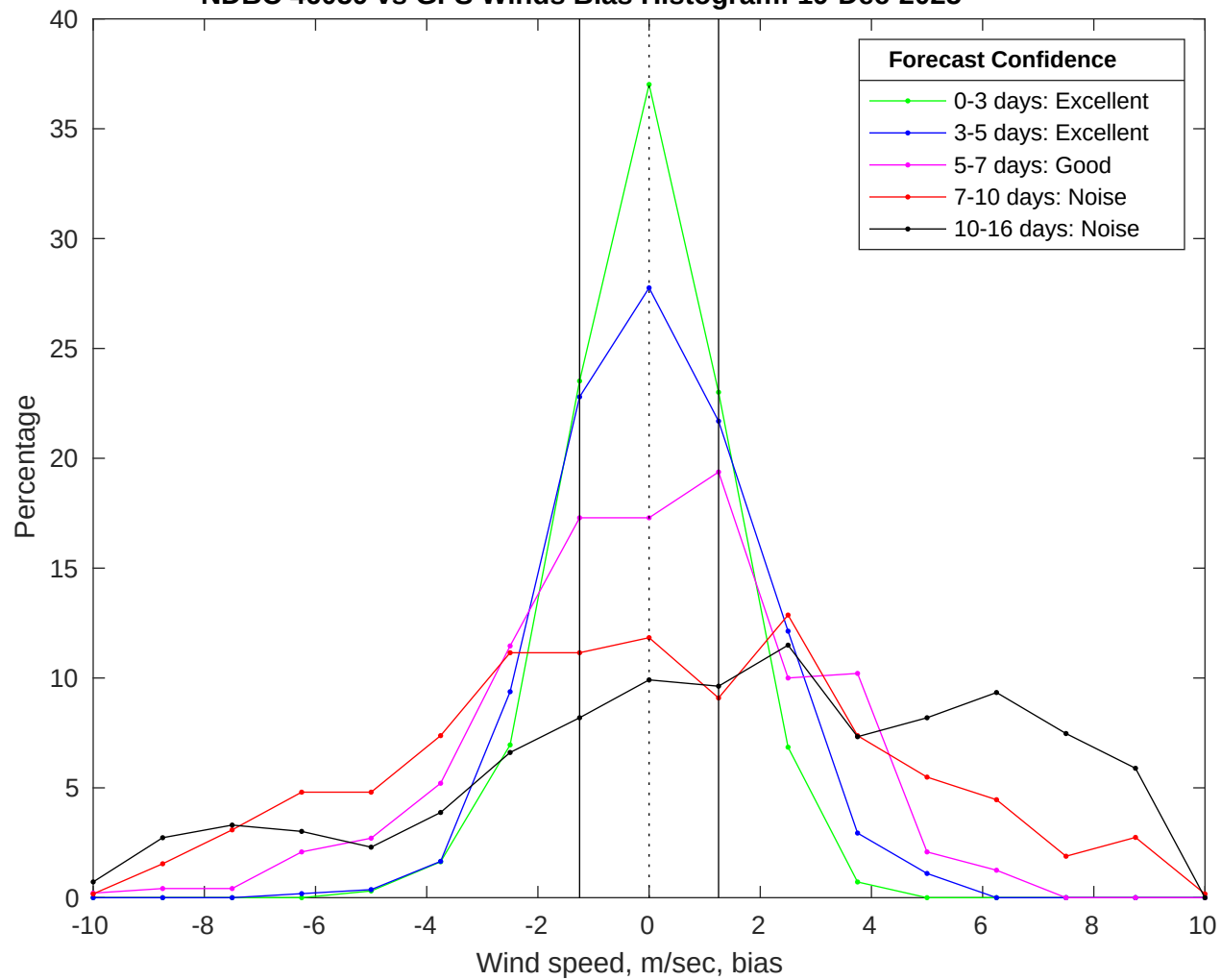
NDBC 46059 vs GFS Winds Bias Histogram: 19-Dec-2025
