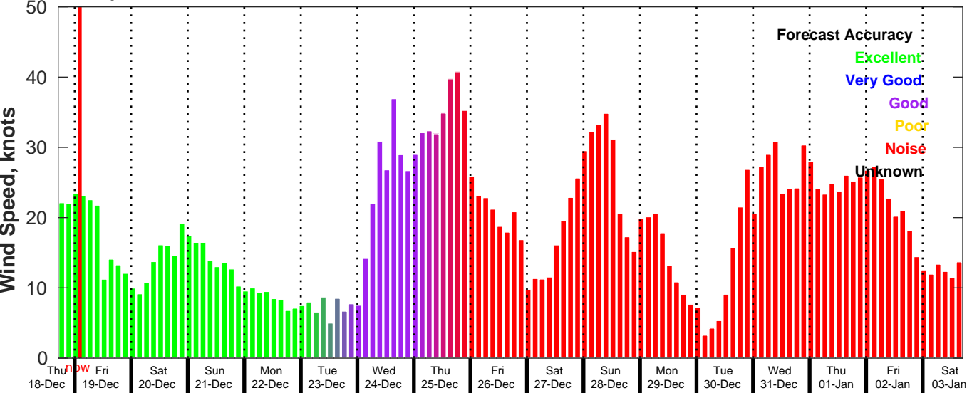
GFS Wind Speed Forecast for NDBC 46059 from 18-Dec-2025 17:00:00 to 03-Jan-2026 17:00:00
