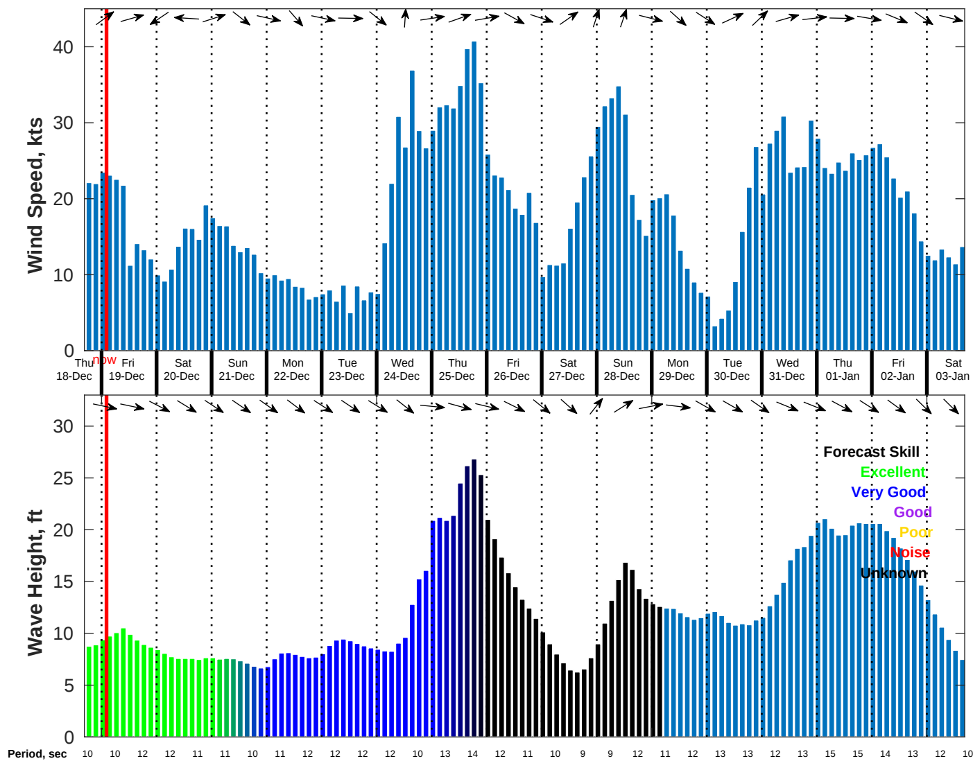
Wind & Wave Forecast for NDBC 46059 from 18-Dec-2025 17:00:00 to 03-Jan-2026 17:00:00
