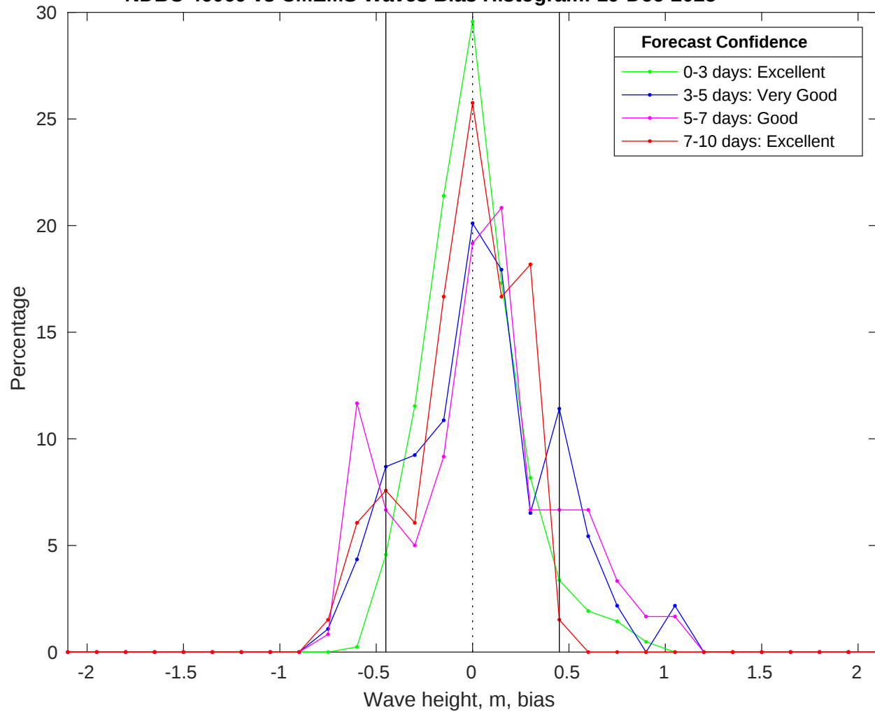
NDBC 46069 vs CMEMS Waves Bias Histogram: 19-Dec-2025
