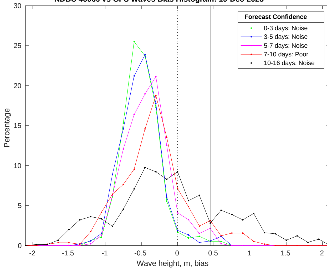
NDBC 46069 vs GFS Waves Bias Histogram: 19-Dec-2025
