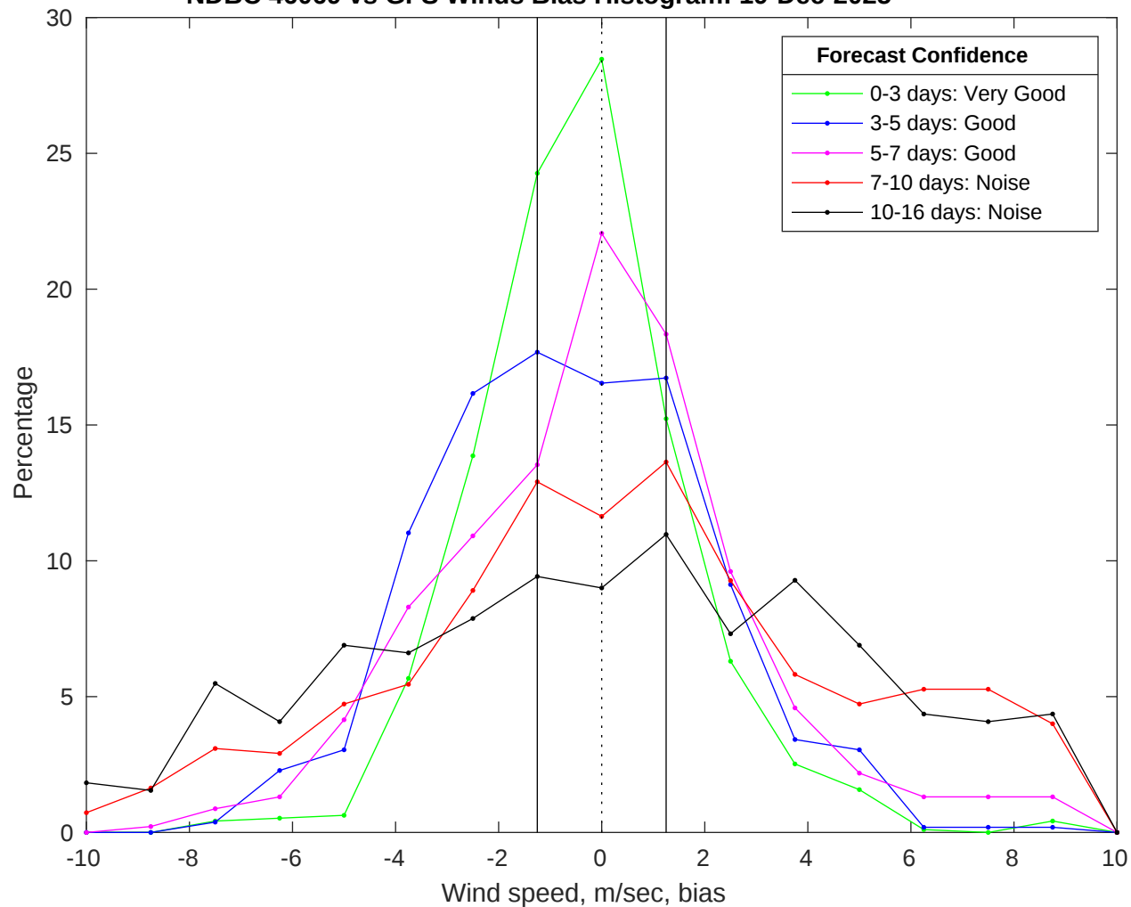
NDBC 46069 vs GFS Winds Bias Histogram: 19-Dec-2025
