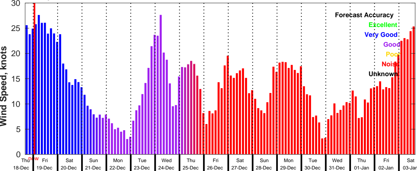
GFS Wind Speed Forecast for NDBC 46069 from 18-Dec-2025 16:00:00 to 03-Jan-2026 16:00:00
