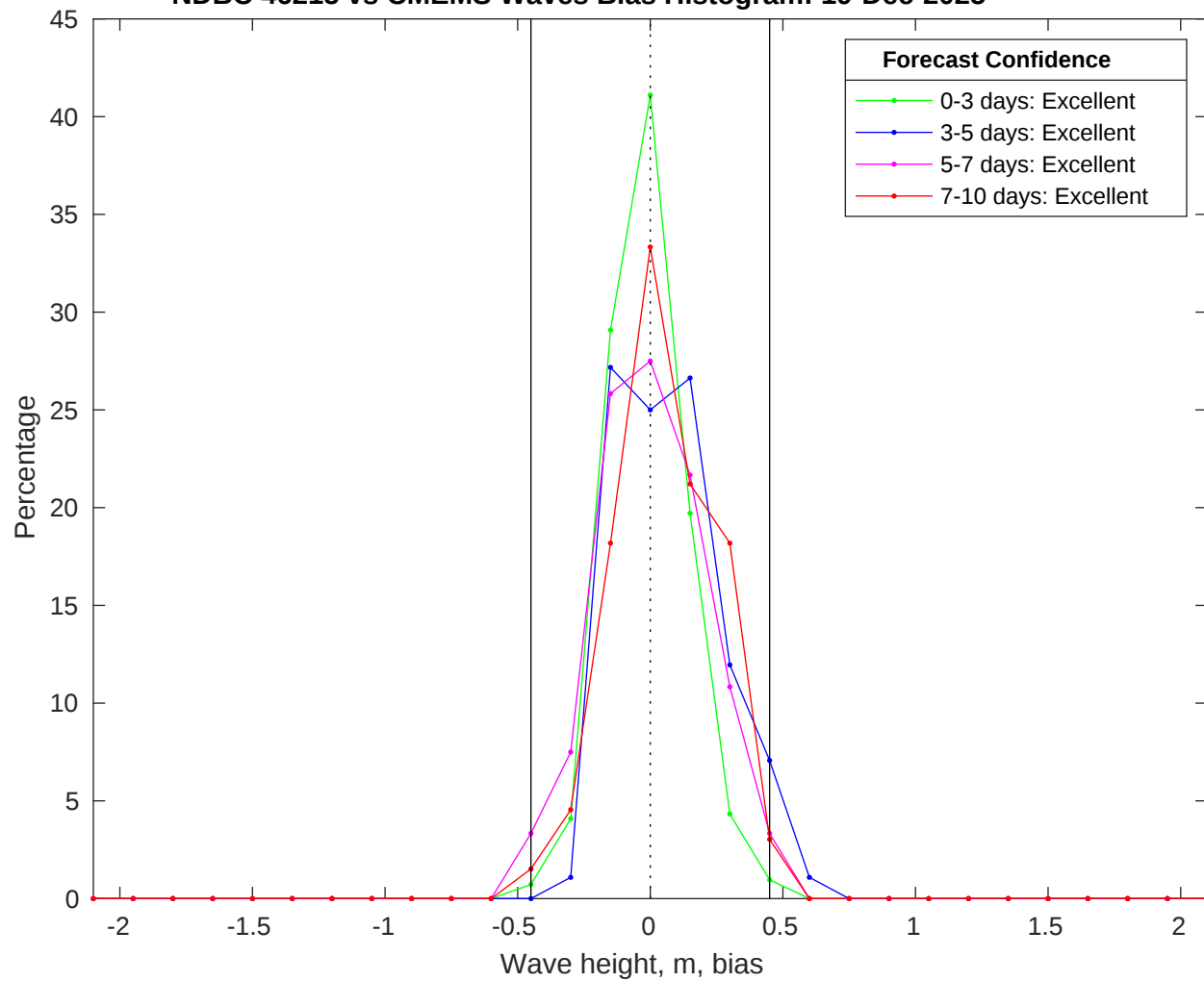
NDBC 46215 vs CMEMS Waves Bias Histogram: 19-Dec-2025
