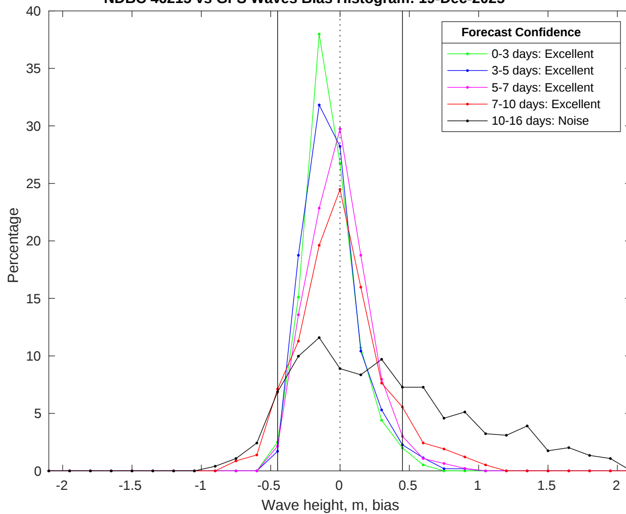
NDBC 46215 vs GFS Waves Bias Histogram: 19-Dec-2025
