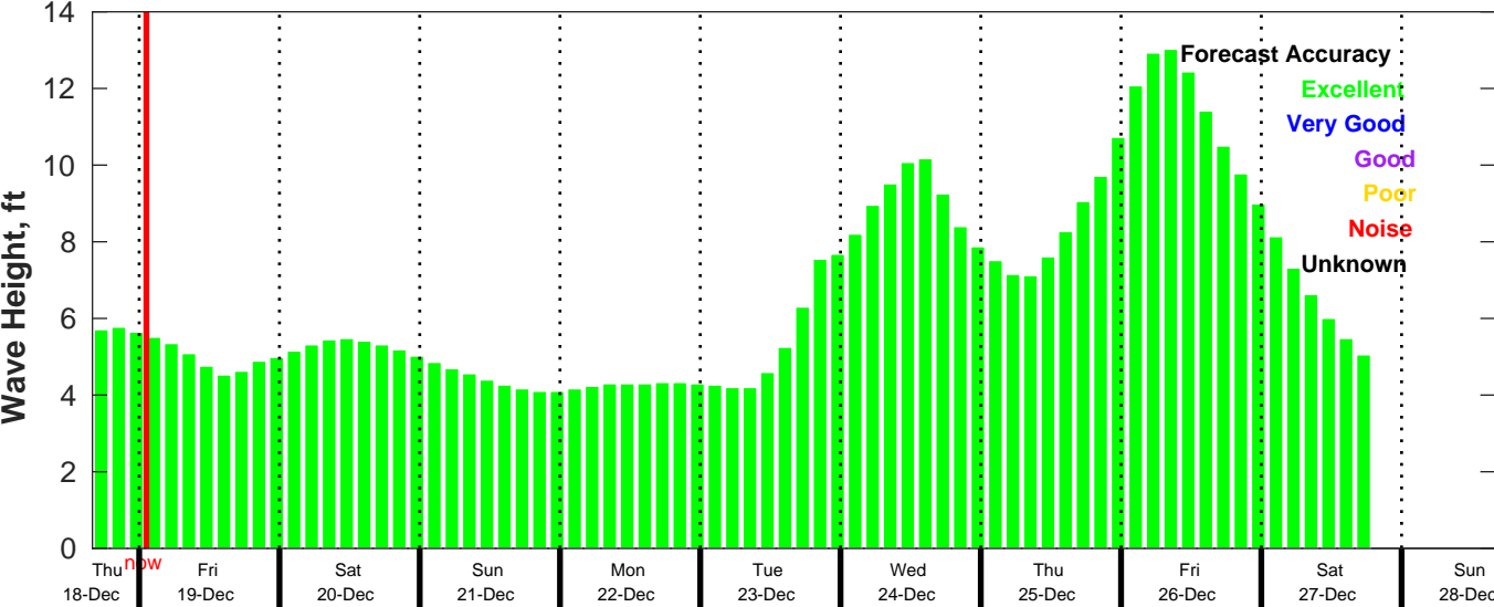
CMEMS Wave Forecast for NDBC 46215 from 18-Dec-2025 16:00:00 to 28-Dec-2025 16:00:00
