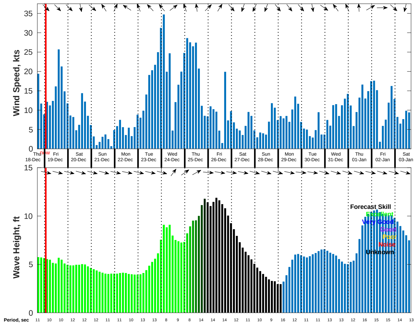
Wind & Wave Forecast for NDBC 46215 from 18-Dec-2025 16:00:00 to 03-Jan-2026 16:00:00
