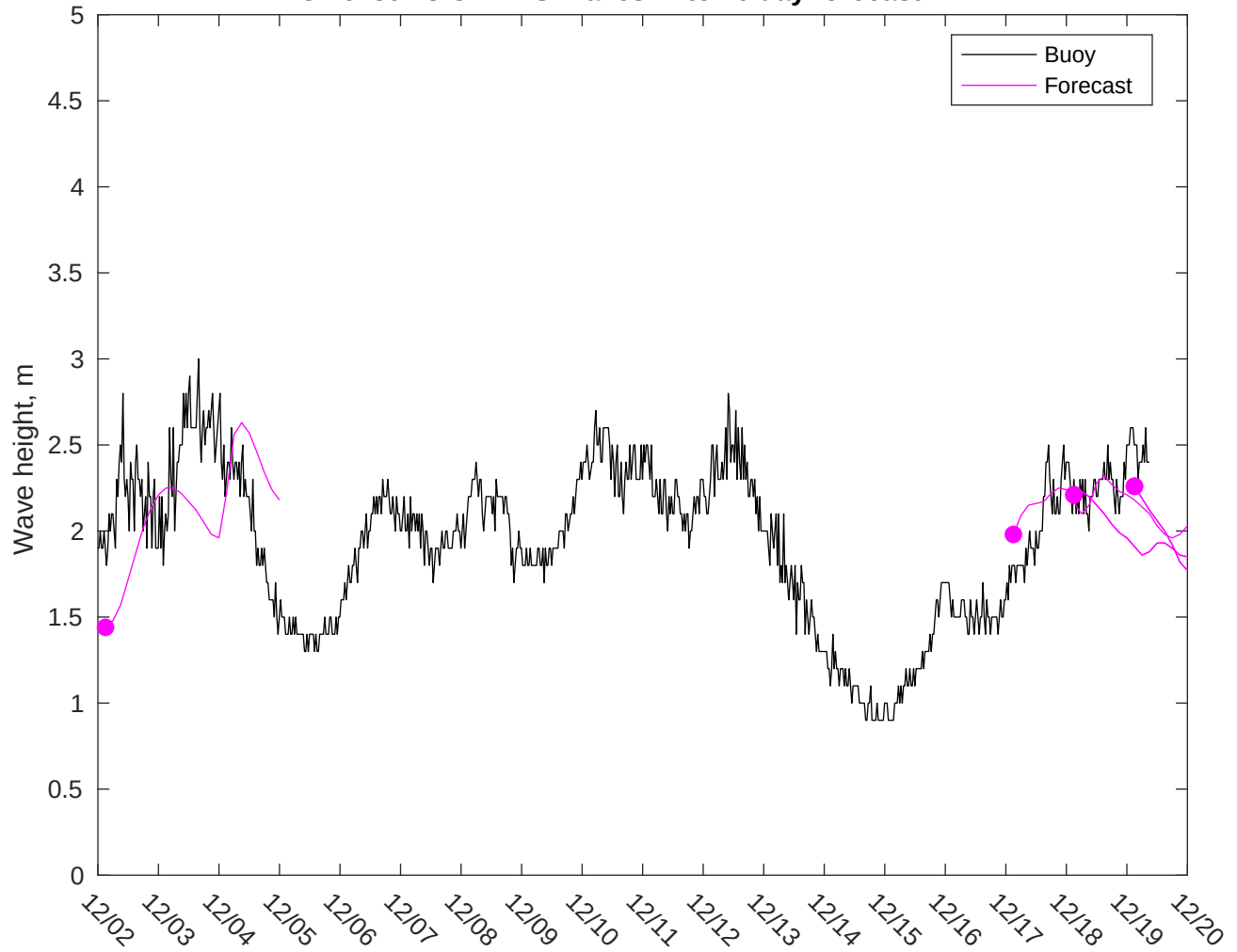
NDBC 46259 vs CMEMS Waves: 7 to 10 day forecast
