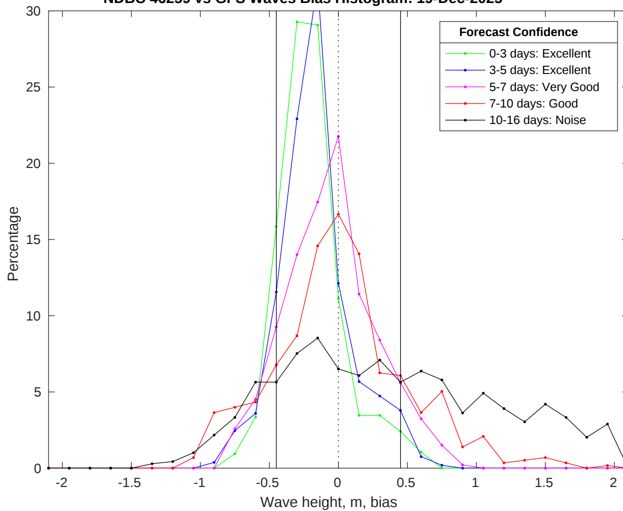
NDBC 46259 vs GFS Waves Bias Histogram: 19-Dec-2025
